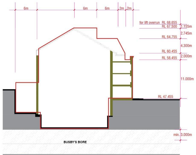
Figure 6.xx: 1-11 Oxford Street, Paddington – Maximum building envelope section
